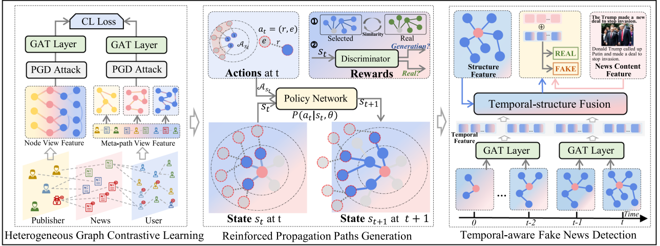
Fig. 2. The overview of proposed RPPG-Fake model. The model includes: (1) Heterogeneous Graph Contrastive Learning for feature extraction, (2) Reinforced Propagation Paths Generation for selecting optimal propagation actions, and (3) Temporal-aware Fake News Detection using fused structural, content, and temporal features. Yellow nodes are publishers, red nodes are news items, and blue nodes are users.
