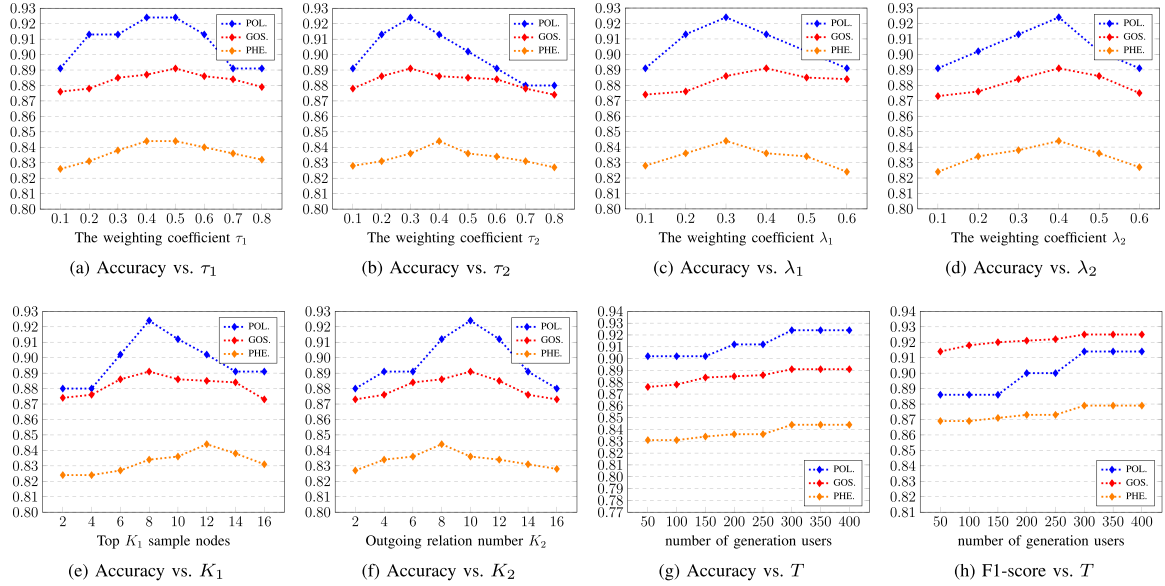
Fig. 4. Parameter Sensitivity Analysis. Impact of different hyperparameters on accuracy and F1-score across three datasets.
